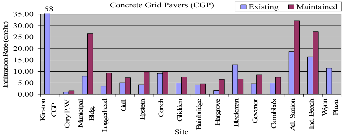
Figure 5. Infiltration rates measured from CGP sites.
