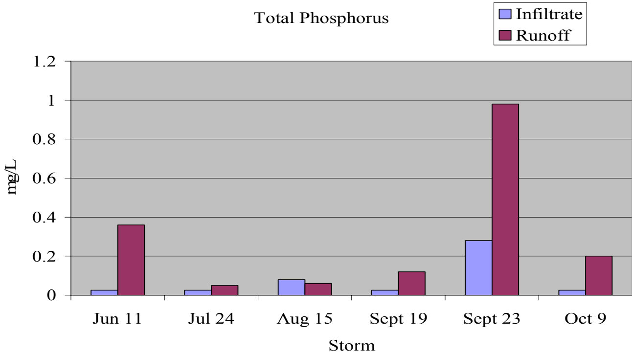
Figure 8. Phosphorus concentrations in runoff and infiltrate from six storms.
