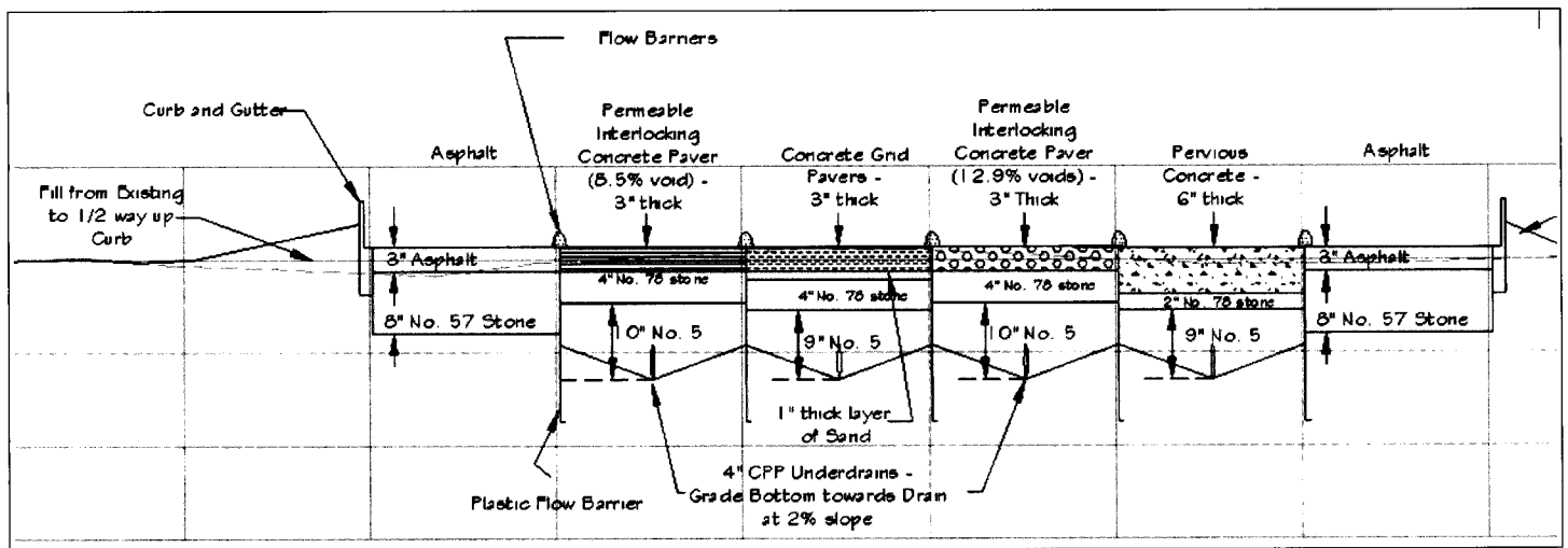
Figure 4. Parking lot cross section showing pavement and base thicknesses in inches (1 inch = 25.4 mm)
