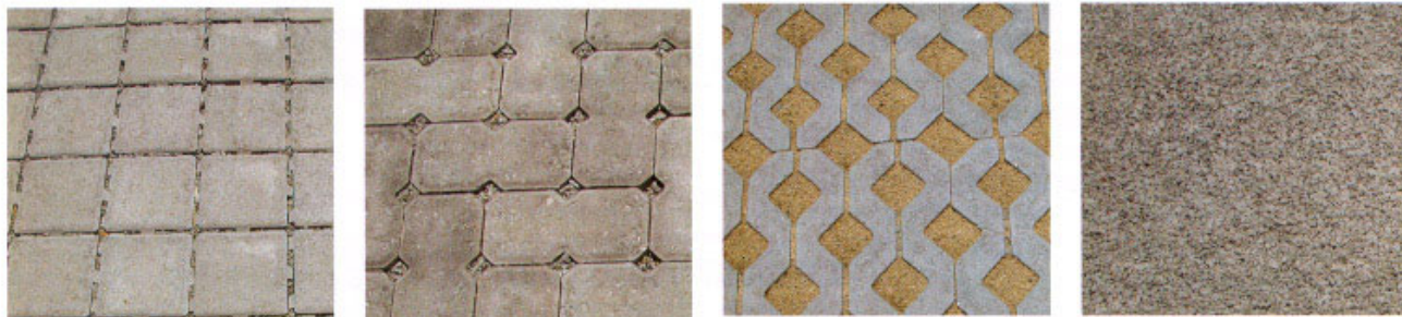
Figure 2. Four runoff-reducing surfaces under evaluation include two types of permeable interlocking concrete pavement with open-graded stone in the openings, concrete grid pavement with sand in the openings and pervious concrete.
