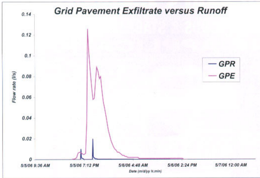
Figure 8. Subsurface exfiltrate is compared to runoff flow for the grid pavement under the same rain event shown in Figure 7. The grids generate a bit more runoff.
