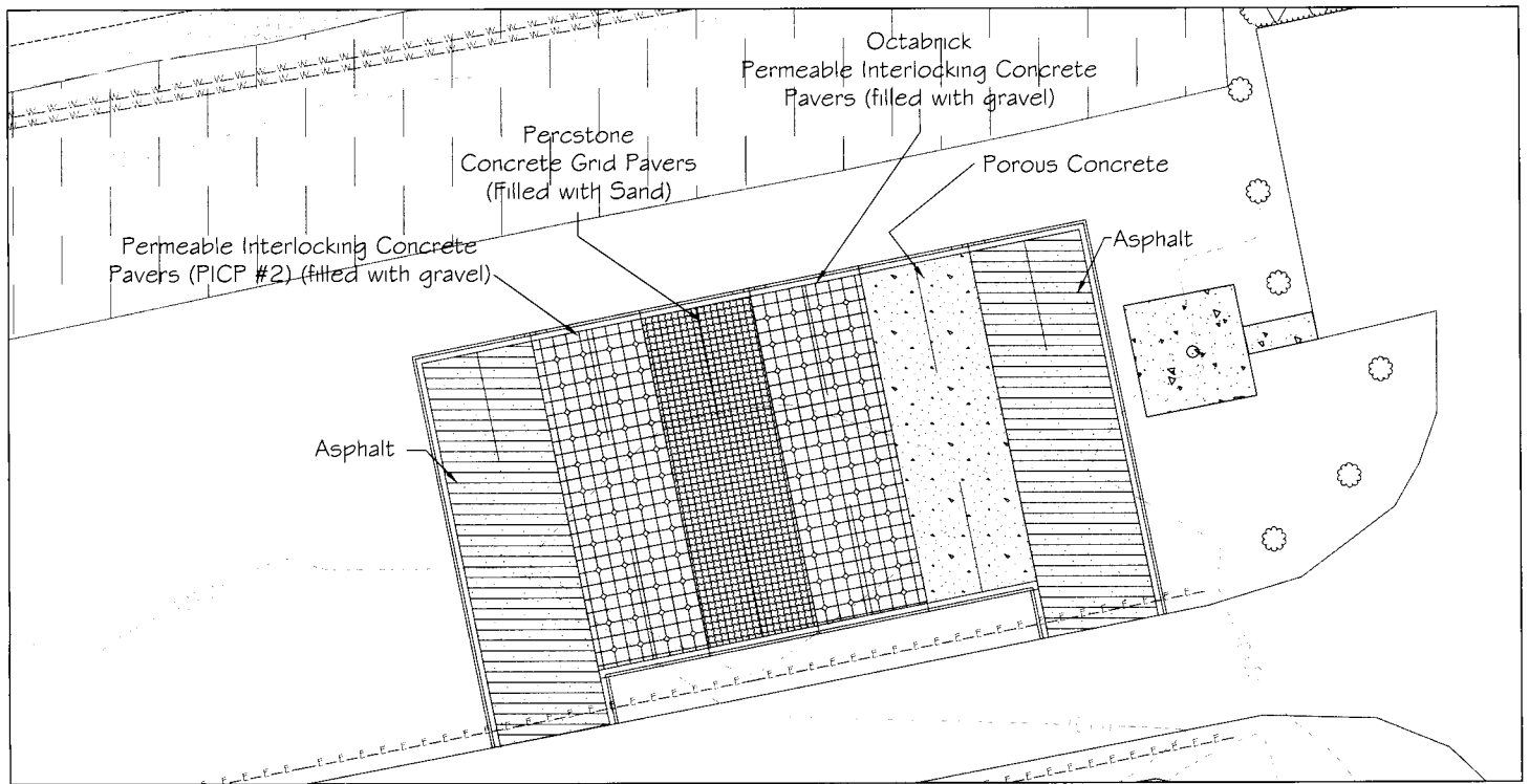
Figure 3. Parking lot plan showing the location of asphalt, pervious (porous) concrete, grid and two permeable interlocking concrete pavements.
