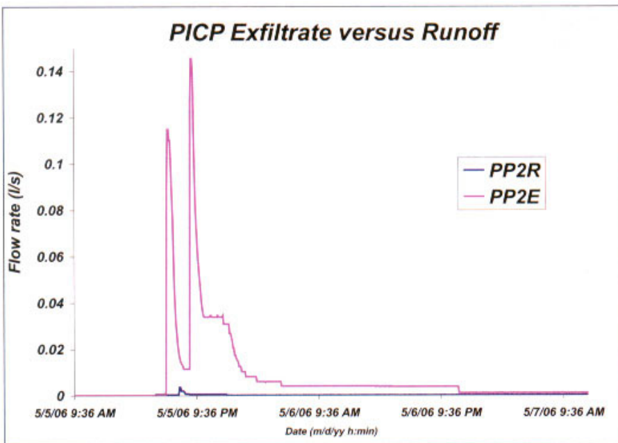
Figure 7. PICP exfiltrate versus runoff hydrograph in early June 2006 for PICP with 8.5% voids
