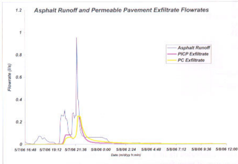
Figure 9. Asphalt runoff versus PICP and pervious concrete exfiltrate flow rates for an early May 2006 rain event
